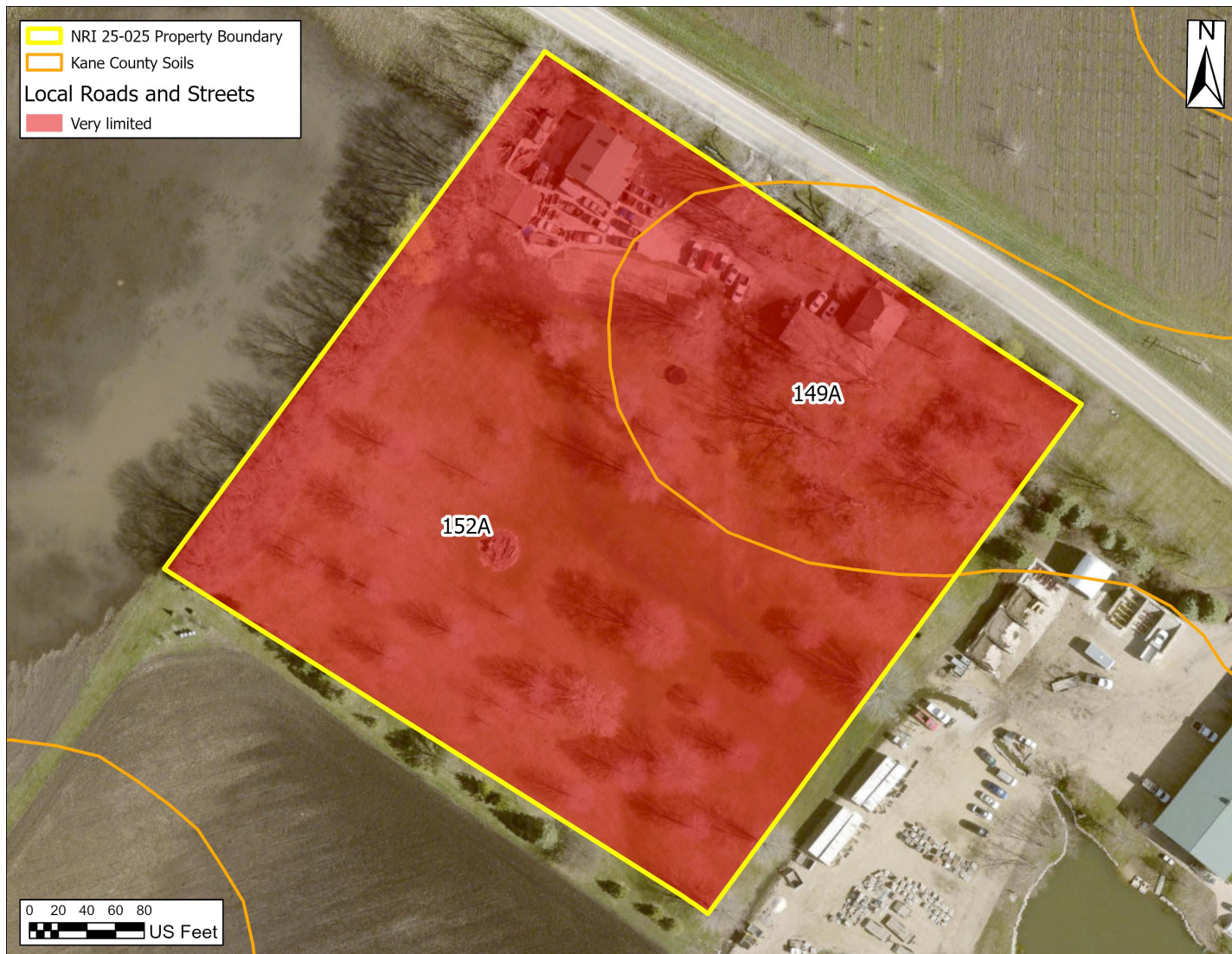
Figure 13: Soil Interpretations for Local Roads and Streets
